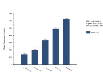
Cytometric bead array sample test of MP51856-1, PFKL Monoclonal Matched Antibody Pair, PBS Only. Capture antibody: 68385-1-PBS. Detection antibody: 68385-2-PBS.
