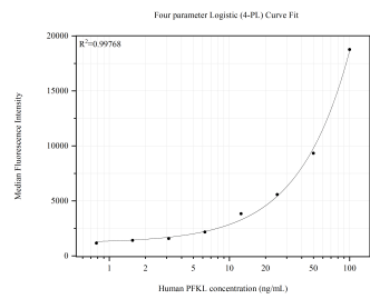
Cytometric bead array standard curve of MP51856-1, PFKL Monoclonal Matched Antibody Pair, PBS Only. Capture antibody: 68385-1-PBS. Detection antibody: 68385-2-PBS. Standard:Ag8250. Range: 0.781-100 ng/mL
