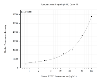
Cytometric bead array standard curve of MP51850-1, CEP135 Monoclonal Matched Antibody Pair, PBS Only. Capture antibody: 68715-1-PBS. Detection antibody: 68715-2-PBS. Standard:Ag19122. Range: 0.781-100 ng/mL
