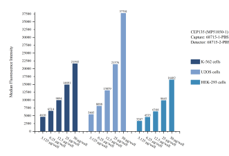
Cytometric bead array sample test of MP51850-1, CEP135 Monoclonal Matched Antibody Pair, PBS Only. Capture antibody: 68715-1-PBS. Detection antibody: 68715-2-PBS.
