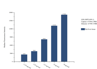
Cytometric bead array sample test of MP51699-1, GSS Monoclonal Matched Antibody Pair, PBS Only. Capture antibody: 67598-2-PBS. Detection antibody: 67598-3-PBS.
