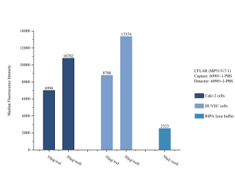
Sample test of MP51317-1, CFLAR Monoclonal Matched Antibody Pair, PBS Only. Capture antibody: 60901-1-PBS. Detection antibody: 60901-2-PBS.
