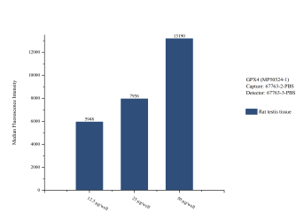
Cytometric bead array sample test of MP50524-1, GPX4 Monoclonal Matched Antibody Pair, PBS Only. Capture antibody: 67763-2-PBS. Detection antibody: 67763-3-PBS.
