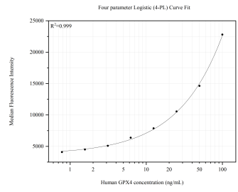
Cytometric bead array standard curve of MP50524-1, GPX4 Monoclonal Matched Antibody Pair, PBS Only. Capture antibody: 67763-2-PBS. Detection antibody: 67763-3-PBS. Standard:Ag30650. Range: 0.781-100 ng/mL.
