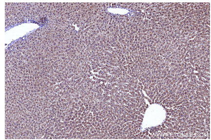
Immunohistochemical analysis of paraffin-embedded rat liver tissue slide using KHC3142 (COX4NB IHC Kit).
