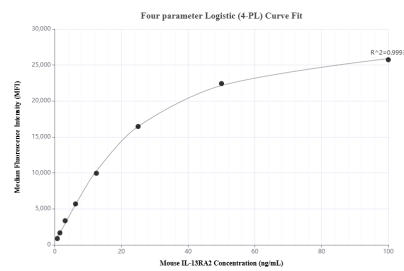
Cytometric bead array standard curve of MP02013-1, MOUSE IL-13RA2 Recombinant Matched Antibody Pair, PBS Only. Capture antibody: 85631-4-PBS. Detection antibody: 85631-2-PBS. Standard: Eg3118. Range: 0.781-100 ng/mL
