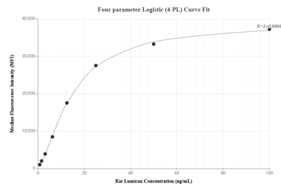
Cytometric bead array standard curve of MP02015-1, RAT Lumican Recombinant Matched Antibody Pair, PBS Only. Capture antibody: 85629-4-PBS. Detection antibody: 85629-2-PBS. Standard: Eg3410. Range: 0.781-100 ng/mL
