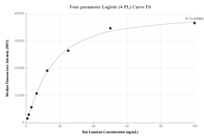
Cytometric bead array standard curve of MP02015-2, RAT Lumican Recombinant Matched Antibody Pair, PBS Only. Capture antibody: 85629-4-PBS. Detection antibody: 85629-3-PBS. Standard: Eg3410. Range: 0.781-100 ng/mL
