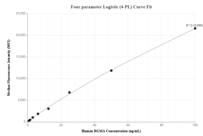
Cytometric bead array standard curve of MP01837-2, RGMA Recombinant Matched Antibody Pair, PBS Only. Capture antibody: 85124-3-PBS. Detection antibody: 85124-1-PBS. Standard: Ag3058. Range: 0.781-100 ng/mL.
