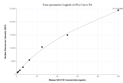
Cytometric bead array standard curve of MP01785-1, MLYCD Recombinant Matched Antibody Pair, PBS Only. Capture antibody: 85080-3-PBS. Detection antibody: 85080-2-PBS. Standard: Ag7334. Range: 0.781-100 ng/mL.
