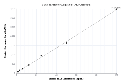
Cytometric bead array standard curve of MP01748-2, TBX5 Recombinant Matched Antibody Pair, PBS Only. Capture antibody: 84997-1-PBS. Detection antibody: 84997-3-PBS. Standard: Ag3845. Range: 1.563-100 ng/mL.
