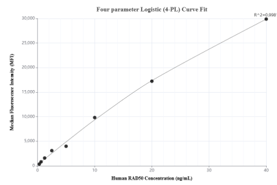
Cytometric bead array standard curve of MP01720-2, RAD50 Recombinant Matched Antibody Pair, PBS Only. Capture antibody: 84969-2-PBS. Detection antibody: 84969-3-PBS. Standard: Ag29949. Range: 0.313-40 ng/mL
