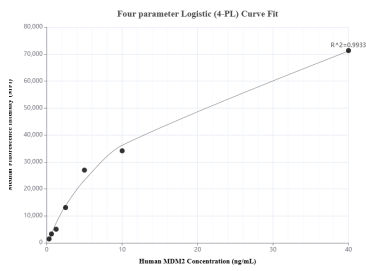
Cytometric bead array standard curve of MP01554-2, MDM2 Recombinant Matched Antibody Pair, PBS Only. Capture antibody: 84780-2-PBS. Detection antibody: 84780-1-PBS. Standard: Ag27255. Range: 0.313-40 ng/mL
