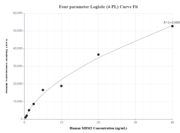
Cytometric bead array standard curve of MP01554-1, MDM2 Recombinant Matched Antibody Pair, PBS Only. Capture antibody: 84780-2-PBS. Detection antibody: 84780-3-PBS. Standard: Ag27255. Range: 0.313-40 ng/mL
