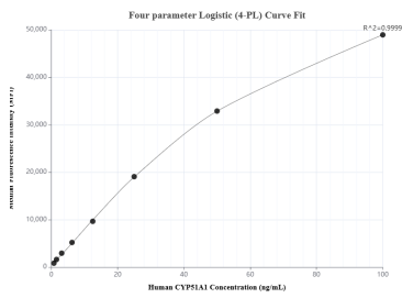
Cytometric bead array standard curve of MP01526-2, CYP51A1 Recombinant Matched Antibody Pair, PBS Only. Capture antibody: 84705-2-PBS. Detection antibody: 84705-3-PBS. Standard: Ag4235. Range: 0.781-100 ng/mL
