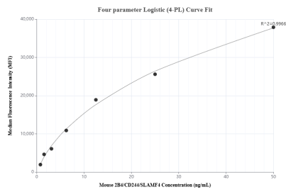
Cytometric bead array standard curve of MP01438-1, MOUSE CD244 Recombinant Matched Antibody Pair, PBS Only. Capture antibody: 84628-2-PBS. Detection antibody: 84628-1-PBS. Standard: Eg1583. Range: 0.781-50 ng/mL
