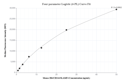
Cytometric bead array standard curve of MP01438-2, MOUSE CD244 Recombinant Matched Antibody Pair, PBS Only. Capture antibody: 84628-3-PBS. Detection antibody: 84628-1-PBS. Standard: Eg1583. Range: 0.781-50 ng/mL
