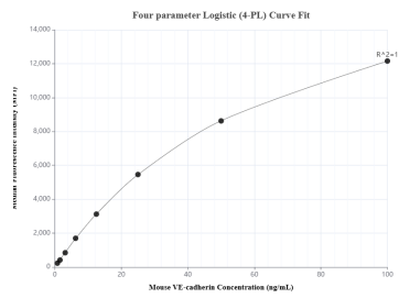
Cytometric bead array standard curve of MP01386-2, MOUSE VE-cadherin/CD144 Recombinant Matched Antibody Pair, PBS Only. Capture antibody: 84529-3-PBS. Detection antibody: 84529-2-PBS. Standard: Eg0921. Range: 0.781-100 ng/mL
