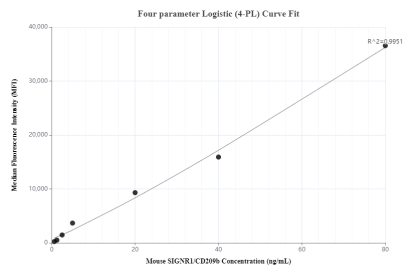
Cytometric bead array standard curve of MP01231-1, MOUSE SIGNR1/CD209b Recombinant Matched Antibody Pair, PBS Only. Capture antibody: 84365-2-PBS. Detection antibody: 84365-3-PBS. Standard: Eg1497. Range: 0.625-80 ng/mL
