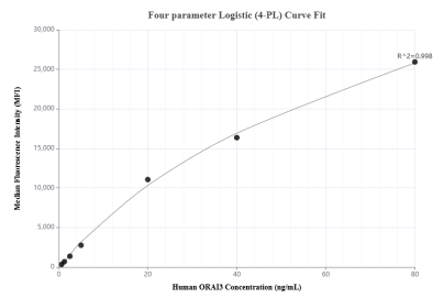
Cytometric bead array standard curve of MP01228-2, ORAI3 Recombinant Matched Antibody Pair, PBS Only. Capture antibody: 84340-1-PBS. Detection antibody: 84340-3-PBS. Standard: Ag36135. Range: 0.625-80 ng/mL
