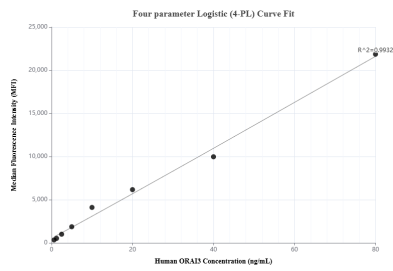
Cytometric bead array standard curve of MP01228-1, ORAI3 Recombinant Matched Antibody Pair, PBS Only. Capture antibody: 84340-3-PBS. Detection antibody: 84340-2-PBS. Standard: Ag36135. Range: 0.625-80 ng/mL
