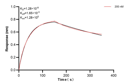
Biolayer interferometry (BLI) kinetic assay of 84292-1-PBS against Human ADAM17 was performed. The affinity constant is 12.8 nM.
