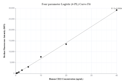
Cytometric bead array standard curve of MP01173-1, CD22 Recombinant Matched Antibody Pair, PBS Only. Capture antibody: 84265-2-PBS. Detection antibody: 84265-3-PBS. Standard: RP02324. Range: 0.313-40 ng/mL
