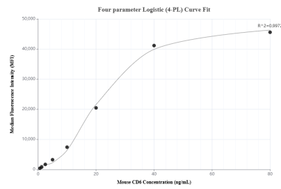
Cytometric bead array standard curve of MP01099-2, MOUSE CD6 Recombinant Matched Antibody Pair, PBS Only. Capture antibody: 84166-3-PBS. Detection antibody: 84166-1-PBS. Standard: Eg1401. Range: 0.625-80 ng/mL
