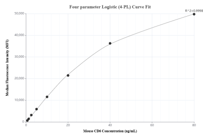
Cytometric bead array standard curve of MP01099-1, MOUSE CD6 Recombinant Matched Antibody Pair, PBS Only. Capture antibody: 84166-2-PBS. Detection antibody: 84166-1-PBS. Standard: Eg1401. Range: 0.625-80 ng/mL
