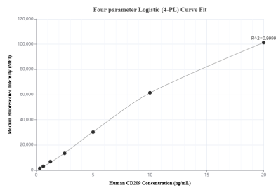
Cytometric bead array standard curve of MP01013-1, CD209 Recombinant Matched Antibody Pair, PBS Only. Capture antibody: 84095-1-PBS. Detection antibody: 84095-2-PBS. Standard: Eg0062. Range: 0.313-20 ng/mL
