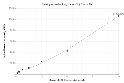
Cytometric bead array standard curve of MP00957-2, REPS2 Recombinant Matched Antibody Pair, PBS Only. Capture antibody: 84016-3-PBS. Detection antibody: 84016-1-PBS. Standard: Ag33764. Range: 0.625-40 ng/mL
