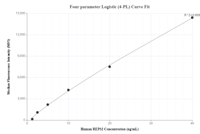
Cytometric bead array standard curve of MP00957-3, REPS2 Recombinant Matched Antibody Pair, PBS Only. Capture antibody: 84016-3-PBS. Detection antibody: 84016-2-PBS. Standard: Ag33764. Range: 1.25-40 ng/mL
