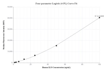
Cytometric bead array standard curve of MP00763-1, IL-33 Recombinant Matched Antibody Pair, PBS Only. Capture antibody: 83765-2-PBS. Detection antibody: 83765-3-PBS. Standard: Eg0313. Range: 1.563-100 ng/mL.
