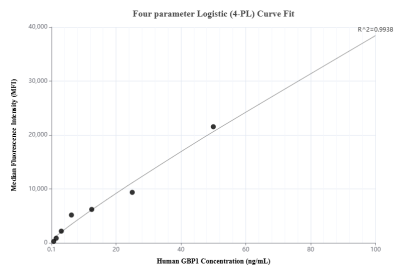
Cytometric bead array standard curve of MP00707-3, GBP1 Recombinant Matched Antibody Pair, PBS Only. Capture antibody: 83751-3-PBS. Detection antibody: 83751-4-PBS. Standard: Ag7562. Range: 0.78-100 ng/mL
