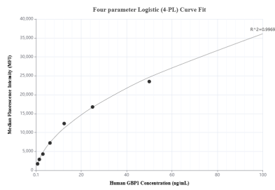
Cytometric bead array standard curve of MP00707-2, GBP1 Recombinant Matched Antibody Pair, PBS Only. Capture antibody: 83751-3-PBS. Detection antibody: 83751-5-PBS. Standard: Ag7562. Range: 0.78-100 ng/mL
