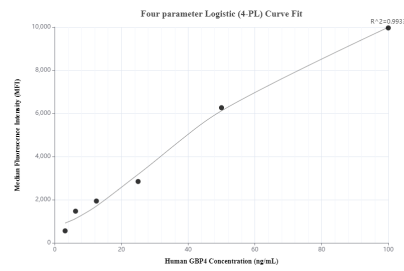
Cytometric bead array standard curve of MP00655-2, GBP4 Recombinant Matched Antibody Pair, PBS Only. Capture antibody: 83699-2-PBS. Detection antibody: 83699-3-PBS. Standard: Ag12006. Range: 3.13-100 ng/mL.
