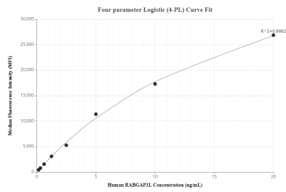
Cytometric bead array standard curve of MP00653-1, RABGAP1L Recombinant Matched Antibody Pair, PBS Only. Capture antibody: 83698-1-PBS. Detection antibody: 83698-2-PBS. Standard: Ag4856. Range: 0.156-20 ng/mL
