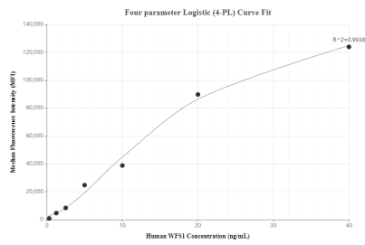
Cytometric bead array standard curve of MP00629-2, WFS1 Recombinant Matched Antibody Pair, PBS Only. Capture antibody: 83642-2-PBS. Detection antibody: 83642-4-PBS. Standard: Ag25735. Range: 0.313-40 ng/mL
