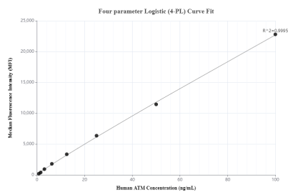
Cytometric bead array standard curve of MP00592-1, ATM Recombinant Matched Antibody Pair, PBS Only. Capture antibody: 83608-1-PBS. Detection antibody: 83608-4-PBS. Standard: Ag25920. Range: 0.781-100 ng/mL.
