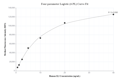
Cytometric bead array standard curve of MP00545-3, IL-2 Recombinant Matched Antibody Pair, PBS Only. Capture antibody: 83558-4-PBS. Detection antibody: 83558-1-PBS. Standard: Eg0828. Range: 0.625-40 ng/mL
