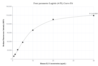
Cytometric bead array standard curve of MP00545-2, IL-2 Recombinant Matched Antibody Pair, PBS Only. Capture antibody: 83558-2-PBS. Detection antibody: 83558-1-PBS. Standard: Eg0828. Range: 0.625-40 ng/mL
