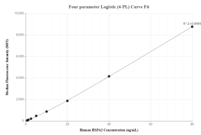
Cytometric bead array standard curve of MP00465-2, HSPA2 Recombinant Matched Antibody Pair, PBS Only. Capture antibody: 83466-1-PBS. Detection antibody: 83466-2-PBS. Standard: Ag3539. Range: 0.625-80 ng/mL
