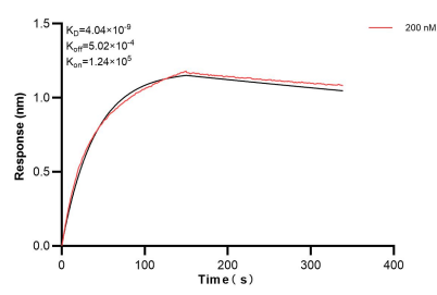
Biolayer interferometry (BLI) kinetic assay of 83465-3-PBS against Human GRIN2A was performed. The affinity constant is 4.04 nM.
