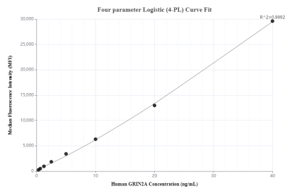
Cytometric bead array standard curve of MP00461-1, GRIN2A Recombinant Matched Antibody Pair, PBS Only. Capture antibody: 83465-3-PBS. Detection antibody: 83465-4-PBS. Standard: Ag29101. Range: 0.313-40 ng/mL
