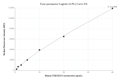
Cytometric bead array standard curve of MP00444-2, TMEM119 Recombinant Matched Antibody Pair, PBS Only. Capture antibody: 83448-1-PBS. Detection antibody: 83448-2-PBS. Standard: Eg0796. Range: 0.625-40 ng/mL
