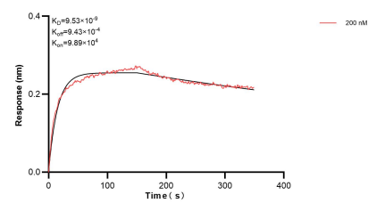
Biolayer interferometry (BLI) kinetic assay of 83448-1-PBS against Human TMEM119 was performed. The affinity constant is 9.53 nM.
