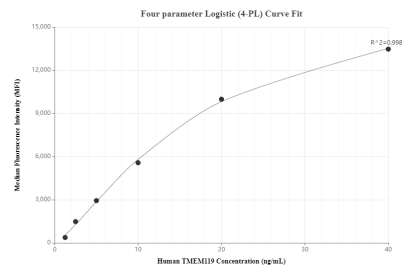
Cytometric bead array standard curve of MP00444-3, TMEM119 Recombinant Matched Antibody Pair, PBS Only. Capture antibody: 83448-1-PBS. Detection antibody: 83448-4-PBS. Standard: Eg0796. Range: 1.25-40 ng/mL
