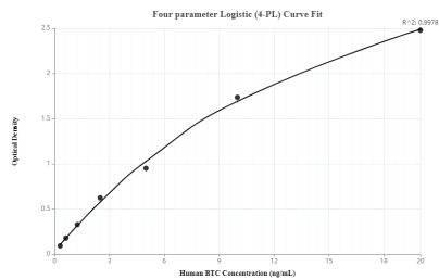
Sandwich ELISA standard curve of MP00138-1, BTC Recombinant Matched Antibody Pair - PBS only. Capture antibody: 83040-3-PBS. Detection antibody: 83040-2-PBS. Standard: Ag26724. Range: 0.313-20 ng/mL
