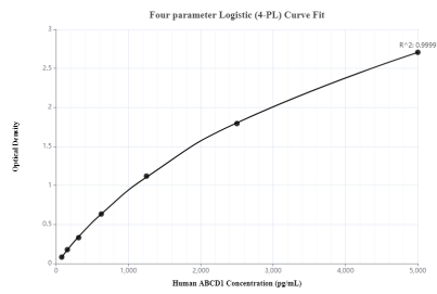
Sandwich ELISA standard curve ofMP00070-1, ABCD1 Recombinant Matched Antibody Pair, PBS Only. Capture antibody: 83038-1-PBS. Detection antibody: 83038-3-PBS. Standard: Ag0453. Range: 78-5000 pg/ mL
