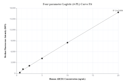
Cytometric bead array standard curve ofMP00070-1, ABCD1 Recombinant Matched Antibody Pair, PBS Only. Capture antibody: 83038-1-PBS. Detection antibody: 83038-3-PBS. Standard: Ag0453. Range: 0.625-20 ng/ mL
