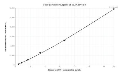
Cytometric bead array standard curve ofMP00115-2, GABRA4 Recombinant Matched Antibody Pair, PBS Only. Capture antibody: 83030-3-PBS. Detection antibody: 83030-2-PBS. Standard: Ag3600. Range: 0.625-20 ng/mL
