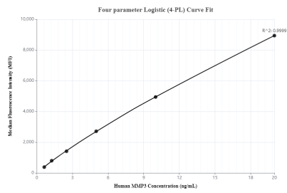
Cytometric bead array standard curve ofMP00083-1, MMP3 Recombinant Matched Antibody Pair, PBS Only. Capture antibody: 82984-1-PBS. Detection antibody: 82984-2-PBS. Standard: Eg0382. Range: 0.625-20 ng/mL
