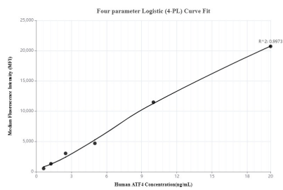
Cytometric bead array standard curve of MP00113-1, ATF4 Recombinant Matched Antibody Pair, PBS Only. Capture antibody: 81798-2-PBS. Detection antibody: 81798-5-PBS. Standard: Ag1279. Range: 0.625-20 ng/mL
