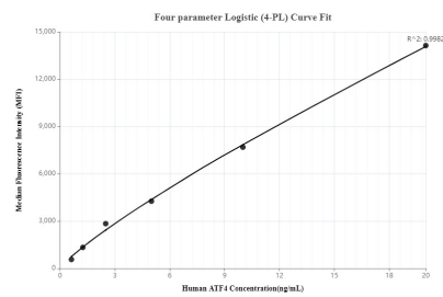
Cytometric bead array standard curve of MP00113-2, ATF4 Recombinant Matched Antibody Pair, PBS Only. Capture antibody: 81798-3-PBS. Detection antibody: 81798-5-PBS. Standard: Ag1279. Range: 0.625-20 ng/mL
