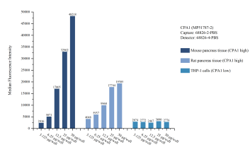
Cytometric bead array sample test of MP51787-2, CPA1 Monoclonal Matched Antibody Pair, PBS Only. Capture antibody: 68826-2-PBS. Detection antibody: 68826-4-PBS.
