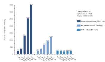
Cytometric bead array sample test of MP51787-1, CPA1 Monoclonal Matched Antibody Pair, PBS Only. Capture antibody: 68826-2-PBS. Detection antibody: 68826-3-PBS.
