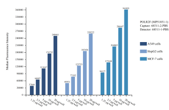
Cytometric bead array sample test of MP51851-1, POLR2F Monoclonal Matched Antibody Pair, PBS Only. Capture antibody: 68511-2-PBS. Detection antibody: 68511-1-PBS.
