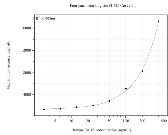
Cytometric bead array standard curve of MP51686-1, ISG15 Monoclonal Matched Antibody Pair, PBS Only. Capture antibody: 68408-2-PBS. Detection antibody: 68408-3-PBS. Standard:Ag8953. Range: 3.125-400 ng/mL.
