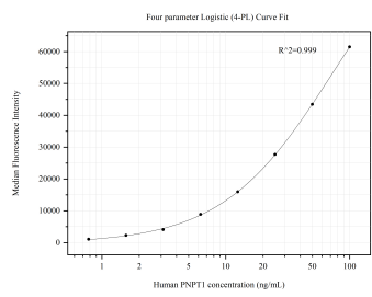
Cytometric bead array standard curve of MP50567-2, PNPT1 Monoclonal Matched Antibody Pair, PBS Only. Capture antibody: 68309-2-PBS. Detection antibody: 68309-4-PBS. Standard:Ag6290. Range: 0.781-100 ng/mL.
