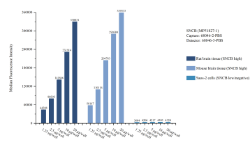
Cytometric bead array sample test of MP51827-1, SNCB Monoclonal Matched Antibody Pair, PBS Only. Capture antibody: 68046-2-PBS. Detection antibody: 68046-3-PBS.
