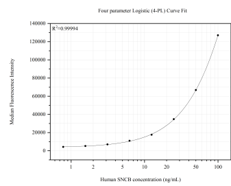
Cytometric bead array standard curve of MP51827-1, SNCB Monoclonal Matched Antibody Pair, PBS Only. Capture antibody: 68046-2-PBS. Detection antibody: 68046-3-PBS. Standard:Ag0772. Range: 0.781-100 ng/mL.
