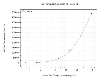
Cytometric bead array standard curve of MP51721-2, PAIP1 Monoclonal Matched Antibody Pair, PBS Only. Capture antibody: 68042-4-PBS. Detection antibody: 68042-5-PBS. Standard: Ag16773. Range: 0.781-50 ng/mL.
