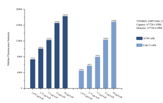
Cytometric bead array sample test of MP51846-1, TXNRD1 Monoclonal Matched Antibody Pair, PBS Only. Capture antibody: 67728-1-PBS. Detection antibody: 67728-2-PBS.
