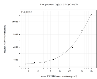
Cytometric bead array standard curve of MP51846-1, TXNRD1 Monoclonal Matched Antibody Pair, PBS Only. Capture antibody: 67728-1-PBS. Detection antibody: 67728-2-PBS. Standard:Ag30071. Range: 0.781-100 ng/mL
