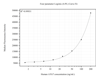
Cytometric bead array standard curve of MP51585-1, ATG7 Monoclonal Matched Antibody Pair, PBS Only. Capture antibody: 67341-3-PBS. Detection antibody: 67341-4-PBS. Standard: Ag29172. Range: 1.563-200 ng/mL.
