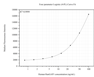
Cytometric bead array standard curve of MP51544-1, RanGAP1 Monoclonal Matched Antibody Pair, PBS Only. Capture antibody: 67146-1-PBS. Detection antibody: 67146-2-PBS. Standard:Ag26136. Range: 0.781-100 ng/mL.
