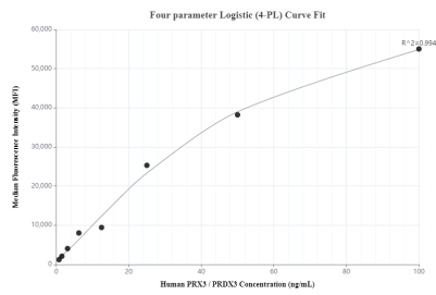
Cytometric bead array standard curve of MP50218-1, PRDX3 Monoclonal Matched Antibody Pair, PBS Only. Capture antibody: 66810-2-PBS. Detection antibody: 66810-3-PBS. Standard: Ag1062. Range: 0.781-100 ng/mL.
