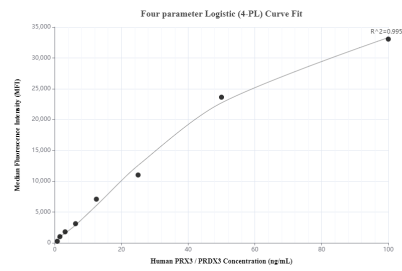
Cytometric bead array standard curve of MP50218-2, PRDX3 Monoclonal Matched Antibody Pair, PBS Only. Capture antibody: 66810-1-PBS. Detection antibody: 66810-2-PBS. Standard: Ag1062. Range: 0.781-100 ng/mL.
