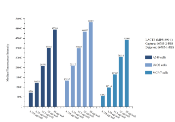
Cytometric bead array sample test of MP51890-1, LACTB Monoclonal Matched Antibody Pair, PBS Only. Capture antibody: 66785-2-PBS. Detection antibody: 66785-1-PBS.
