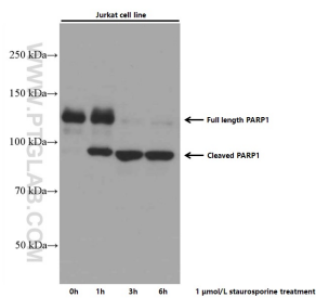
Jurkat cells (20 μ g/lane) treated with staurosporine were subjected to SDS PAGE followed by western blot with 66520-1-Ig (PARP1 antibody) at dilution of 1:40000 incubated at room temperature for 1.5 hours.
